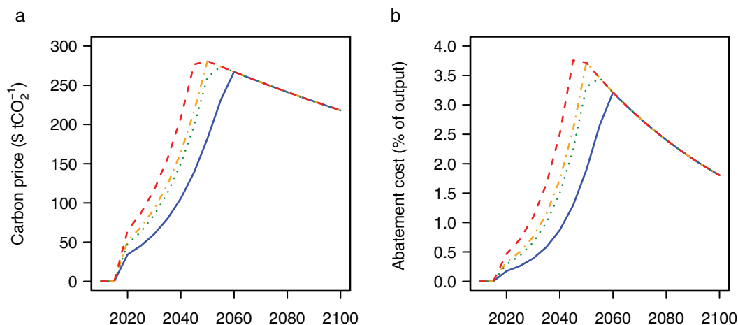
Figure 3. Economic implications. (a) Carbon price. (b) Abatement cost (percentage of output). The yellow line (dash-dotted) describes a stabilization process after 2050 ( 2^{\circ}\text{C\_SIAF\_Stabilization} ). The blue line (solid) at zero radiative forcing refers to the baseline scenario without SIAF mechanism ( 2^{\circ}\text{C} ). The green line (dotted) describes a partial recovery process ( 2^{\circ}\text{C\_SIAF\_Recovery} ) and the red line (dashed) assumes a continued loss of sea ice ( 2^{\circ}\text{C\_SIAF\_No-Recovery} ).
